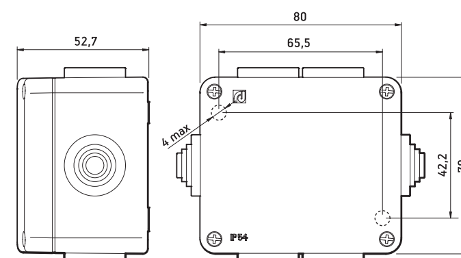
Razvodna kutija Junction box
