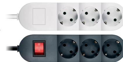
Priključnica prenosna nerastavna trostruka, max 3600W, 3x16A 250V- Triple portable socket outlet unwireable, max 3600W, 3x16A 250V-
