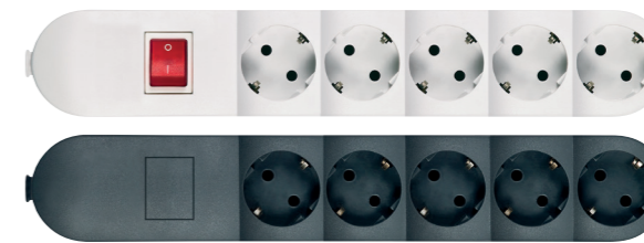
4405.x Priključnica prenosna petostruka, bez kabl, sa dvopolnom indikatorskom sklopkom. max 3600W, 5x16A 250V- Fivefold portable socket outlet, without cord, with double-pole indication switch, max 3600W, 5x16A 250V-
