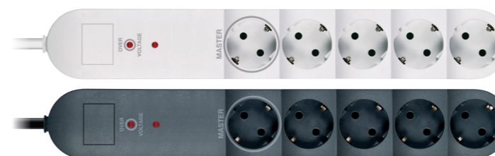
Priključnica prenosna nerastavna petostruka, sa prenaponskom zaštitom, bez sklopke. max 3600W, 5x16A 250V- Fivefold portable socket outlet unwireable, with surge protection, without switch, max 3600W, 5x16A 250V-
