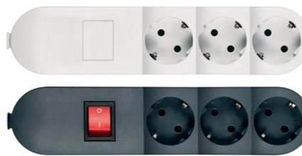
4403.x Priključnica prenosna trostruka, bez kabl, sa dvopolnom indikatorskom sklopkom. max 3600W, 3x16A 250V- Triple portable socket outlet, without cord, with double-pole indication switch, max 3600W, 3x16A 250V-
