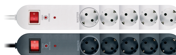
44601.x sa dvopolnom indikatorskom sklopkom with double-pole indication switch 44801.x sa prenaponskom zaštitom klase III, Up<1,5kV, RFI/EMI filterom i prenaponskim filterom za telefon/modem/fax liniju with surge protection class III, Up<1,5kV, RFI/EMI filter and surge filter for phone/modem/fax line 44901.x sa prenaponskom zaštitom klase III, Up<1,5kV i 1+4 MASTER-SLAVE (snaga uključena SLAVE priključnice min 15W) with surge protection class III, Up<1,5kV and 1+4 MASTER-SLAVE (switching threshold min 15W)
