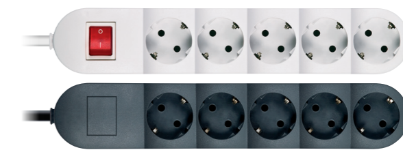
Priključnica prenosna nerastavna petostruka, max 3600W, 5x16A 250V~ Fivefold portable socket outlet unwireable, max 3600W, 5x16A 250V~
