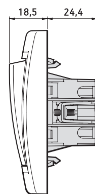
Sklopke Switches
