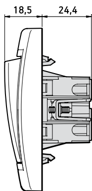
Sklopke Switches
