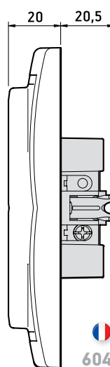
Osnova maske 80 x 123 mm Cover frame base 80 x 123 mm
